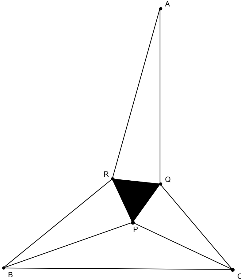
Construction #1 of Morley's Trisector Theorem
